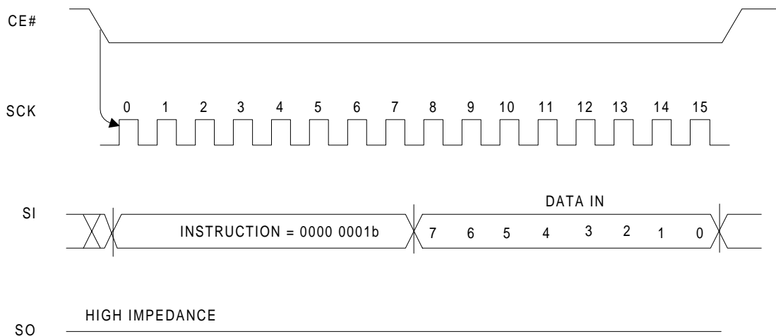
Figure 8. Write Status Register Sequence
