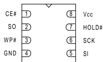
8-Contact WSON
